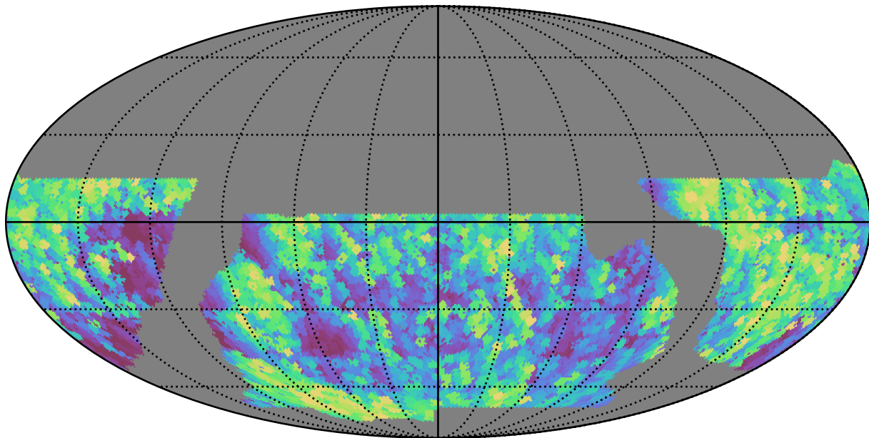
baseline_v2.1_10yrs WFD all bands: Max airmass
