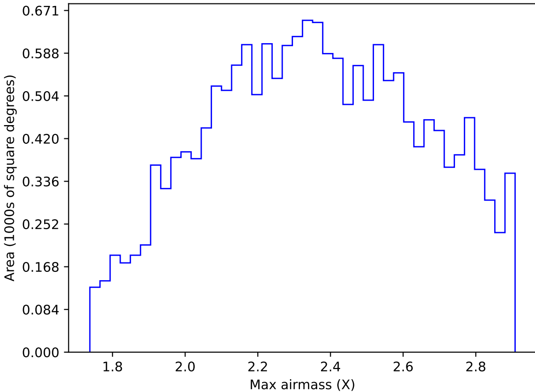
baseline_v2.1_10yrs WFD all bands: Max airmass
