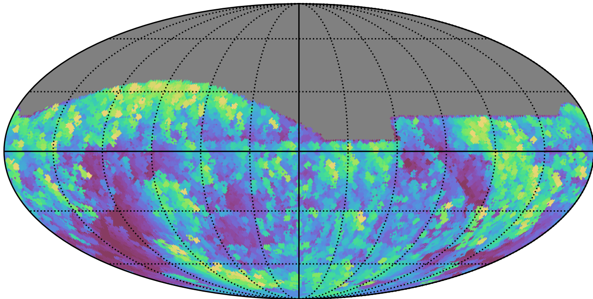
baseline_v2.1_10yrs All sky z band: Max airmass
