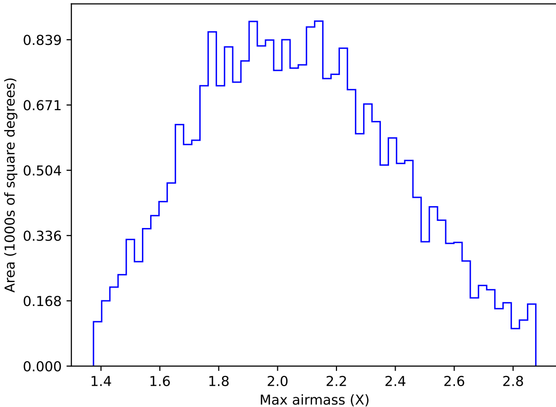
baseline_v2.1_10yrs All sky z band: Max airmass
