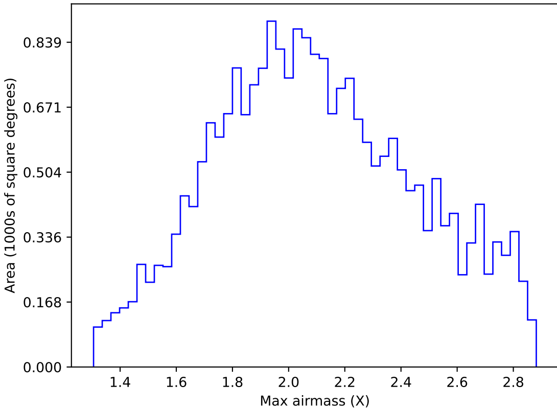
baseline_v2.1_10yrs All sky y band: Max airmass
