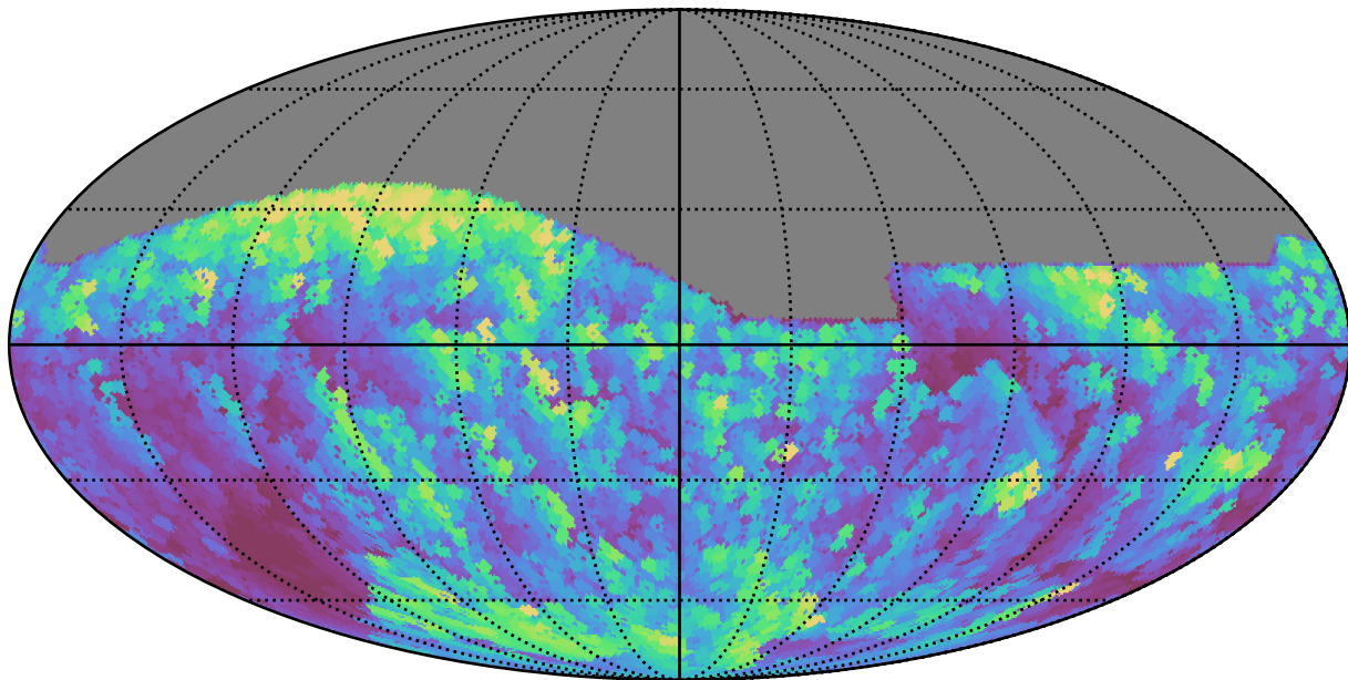
baseline_v2.1_10yrs All sky r band: Max airmass
