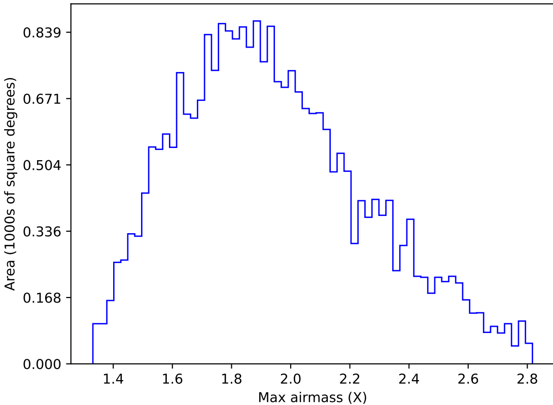
baseline_v2.1_10yrs All sky r band: Max airmass
