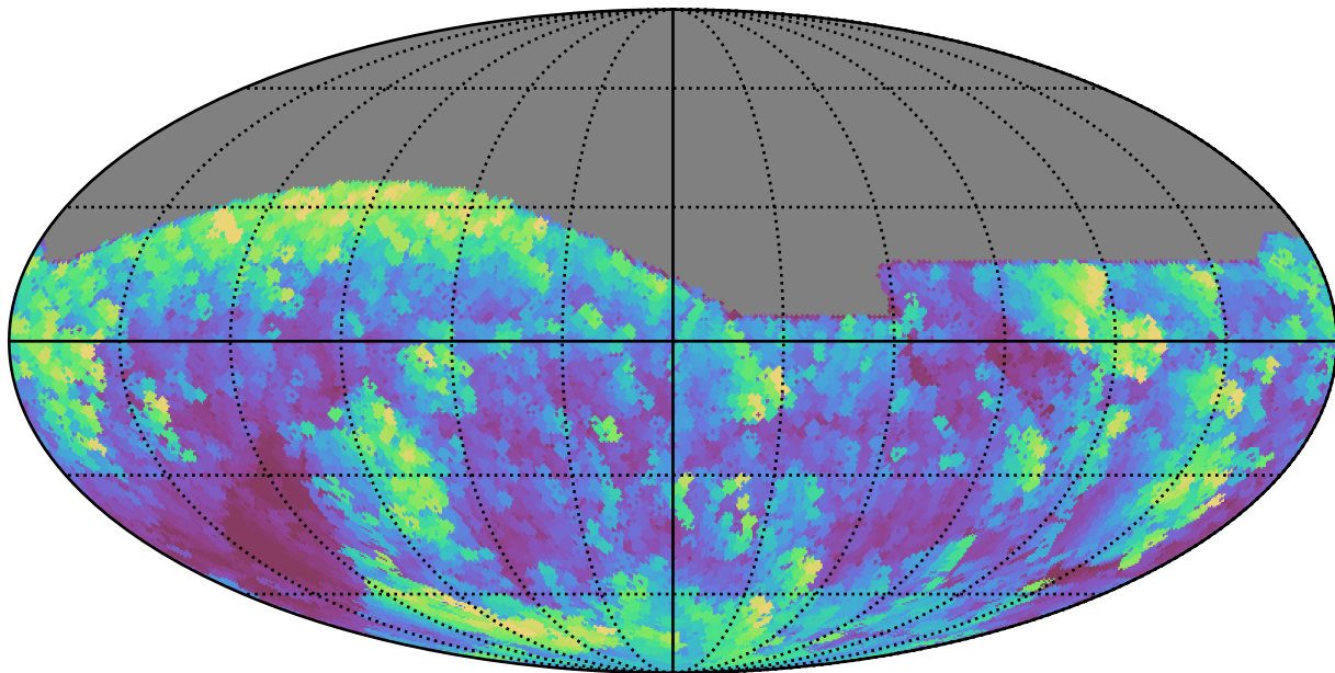
baseline_v2.1_10yrs All sky i band: Max airmass
