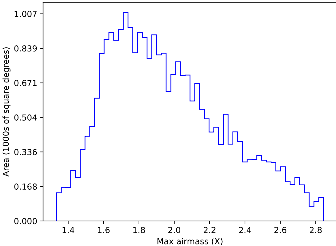
baseline_v2.1_10yrs All sky i band: Max airmass
