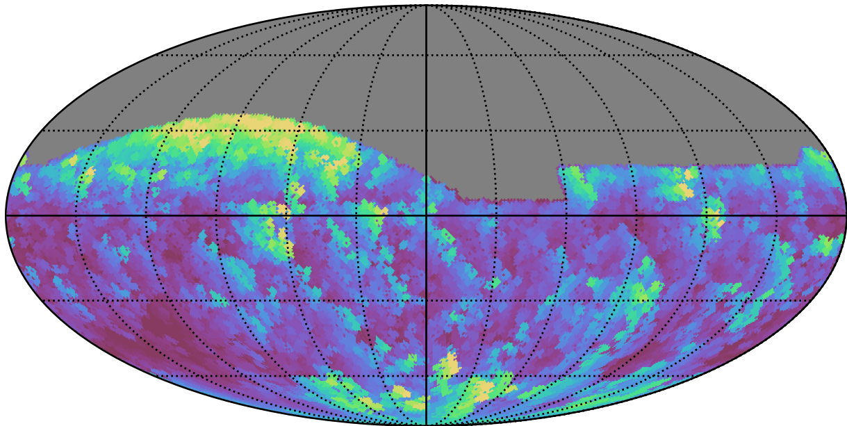
baseline_v2.1_10yrs All sky g band: Max airmass
