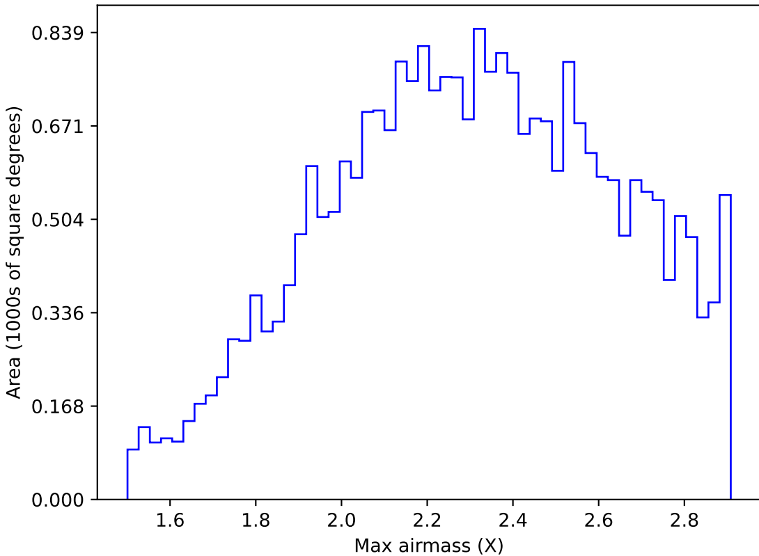
baseline_v2.1_10yrs All sky all bands: Max airmass
