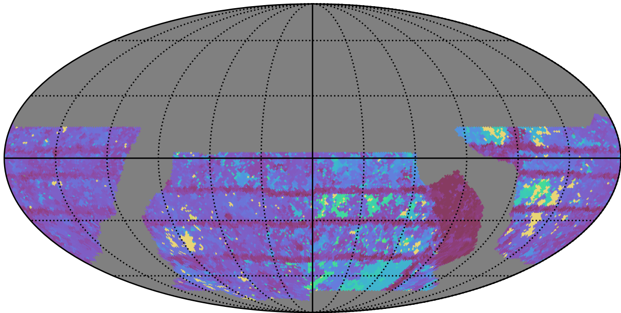
baseline_v2.1_10yrs WFD z band: Max Inter-Night Gap
