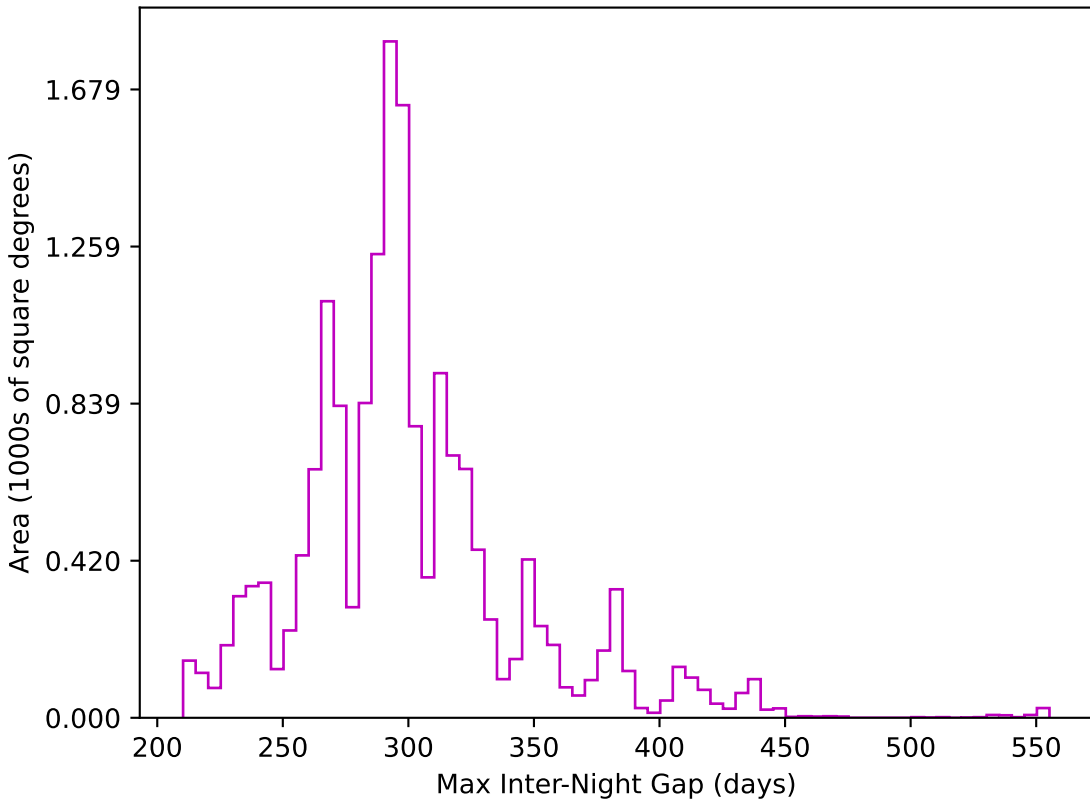
baseline_v2.1_10yrs WFD z band: Max Inter-Night Gap
