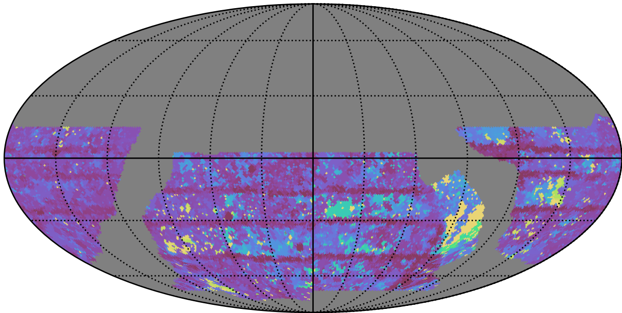
baseline_v2.1_10yrs WFD y band: Max Inter-Night Gap
