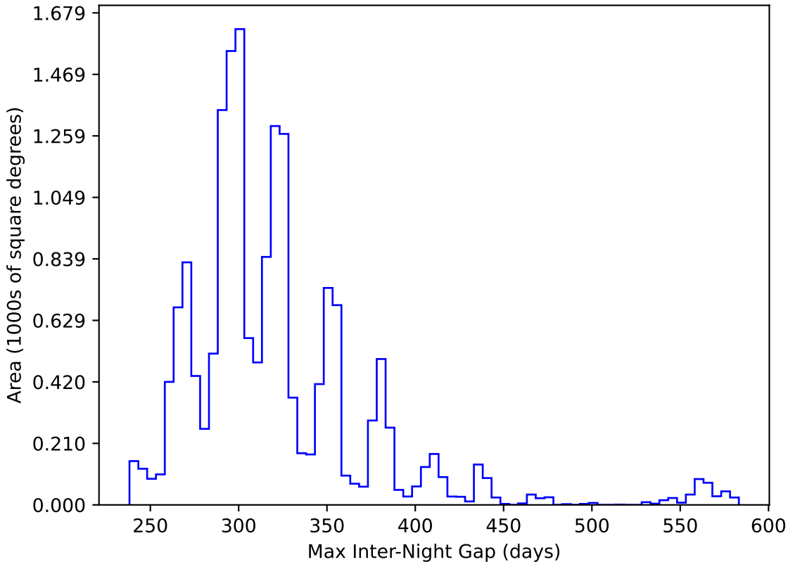
baseline_v2.1_10yrs WFD y band: Max Inter-Night Gap
