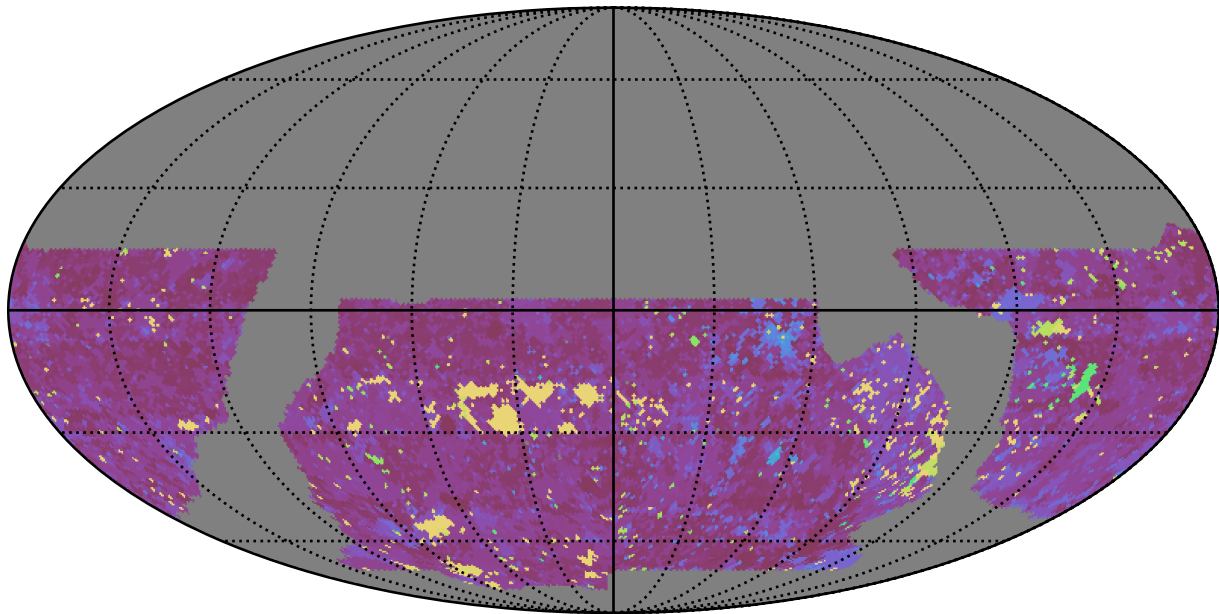
baseline_v2.1_10yrs WFD u band: Max Inter-Night Gap
