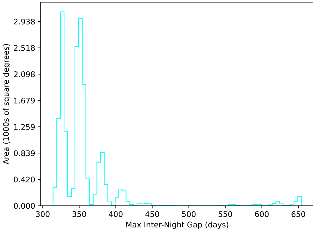
baseline_v2.1_10yrs WFD u band: Max Inter-Night Gap
