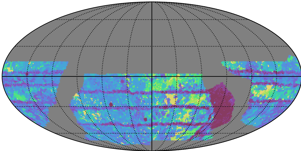
baseline_v2.1_10yrs WFD r band: Max Inter-Night Gap
