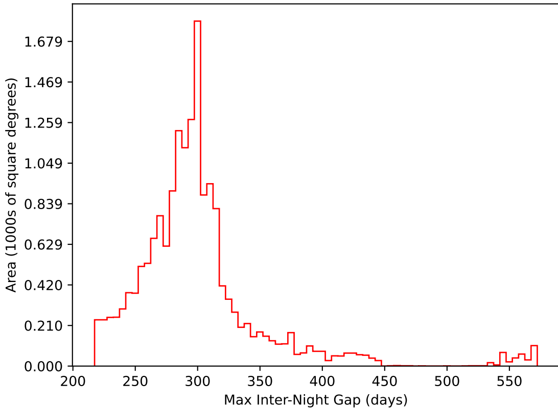
baseline_v2.1_10yrs WFD i band: Max Inter-Night Gap
