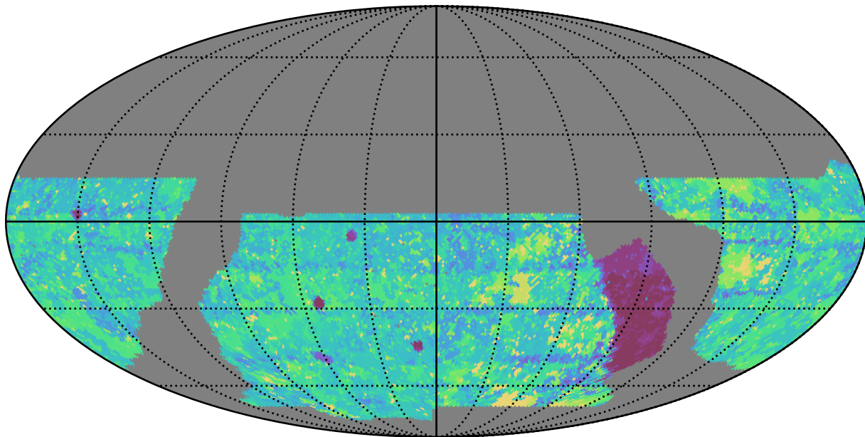
baseline_v2.1_10yrs WFD g band: Max Inter-Night Gap
