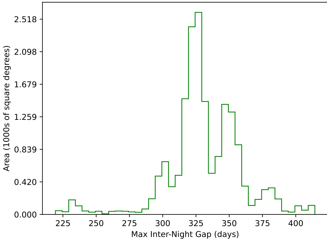
baseline_v2.1_10yrs WFD g band: Max Inter-Night Gap
