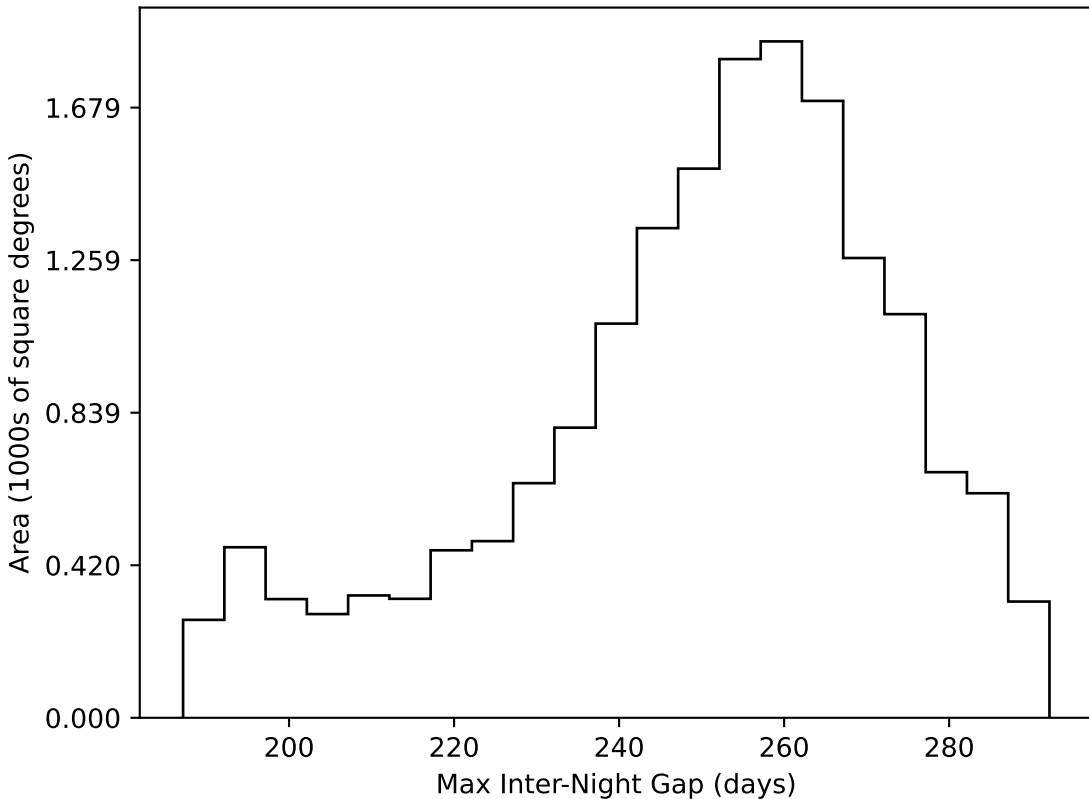
baseline_v2.1_10yrs WFD all bands: Max Inter-Night Gap
