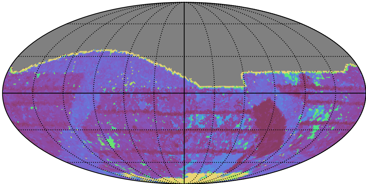
baseline_v2.1_10yrs All sky z band: Max Inter-Night Gap
