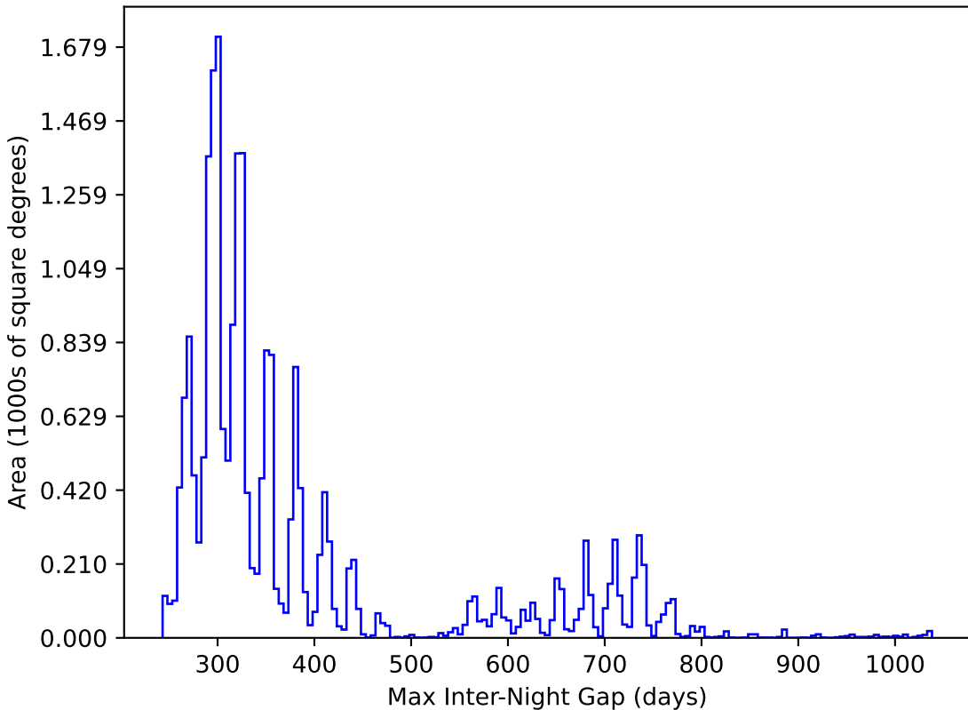
baseline_v2.1_10yrs All sky y band: Max Inter-Night Gap
