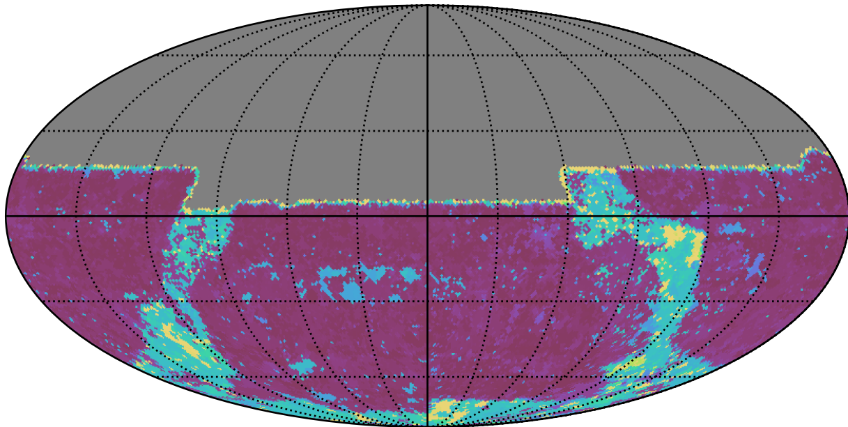
baseline_v2.1_10yrs All sky u band: Max Inter-Night Gap
