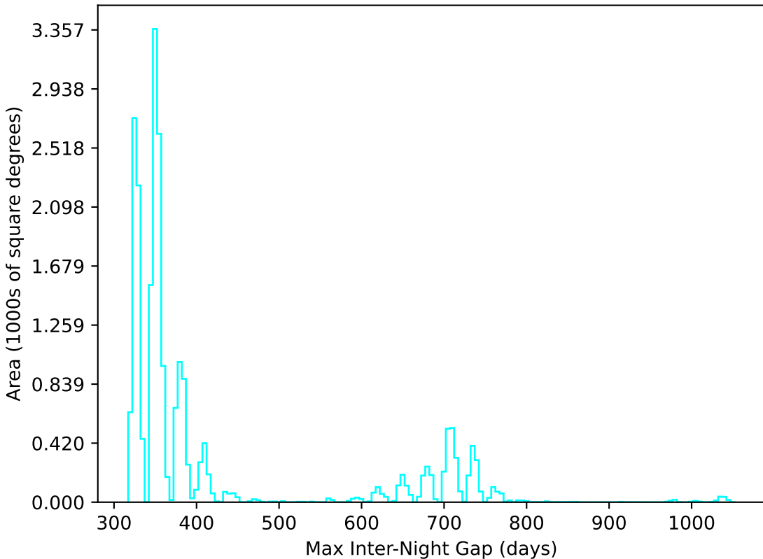
baseline_v2.1_10yrs All sky u band: Max Inter-Night Gap
