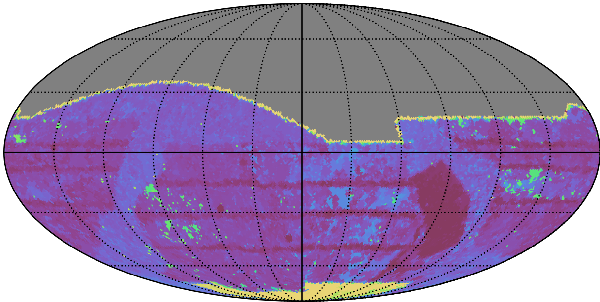
baseline_v2.1_10yrs All sky r band: Max Inter-Night Gap
