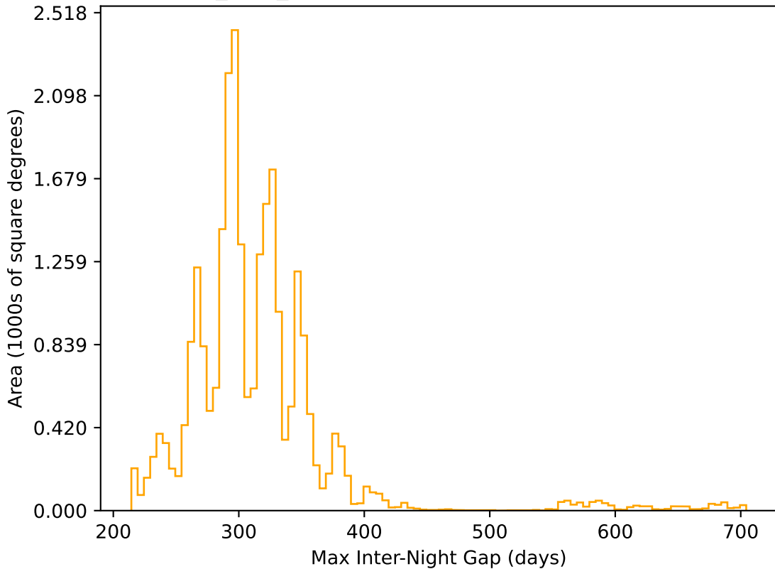
baseline_v2.1_10yrs All sky r band: Max Inter-Night Gap
