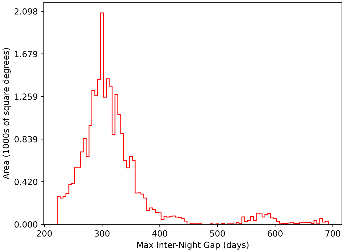
baseline_v2.1_10yrs All sky i band: Max Inter-Night Gap
