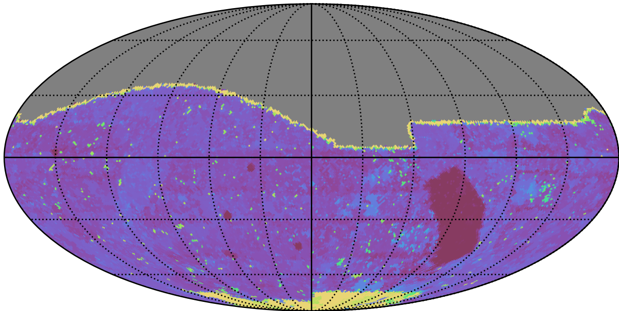
baseline_v2.1_10yrs All sky g band: Max Inter-Night Gap
