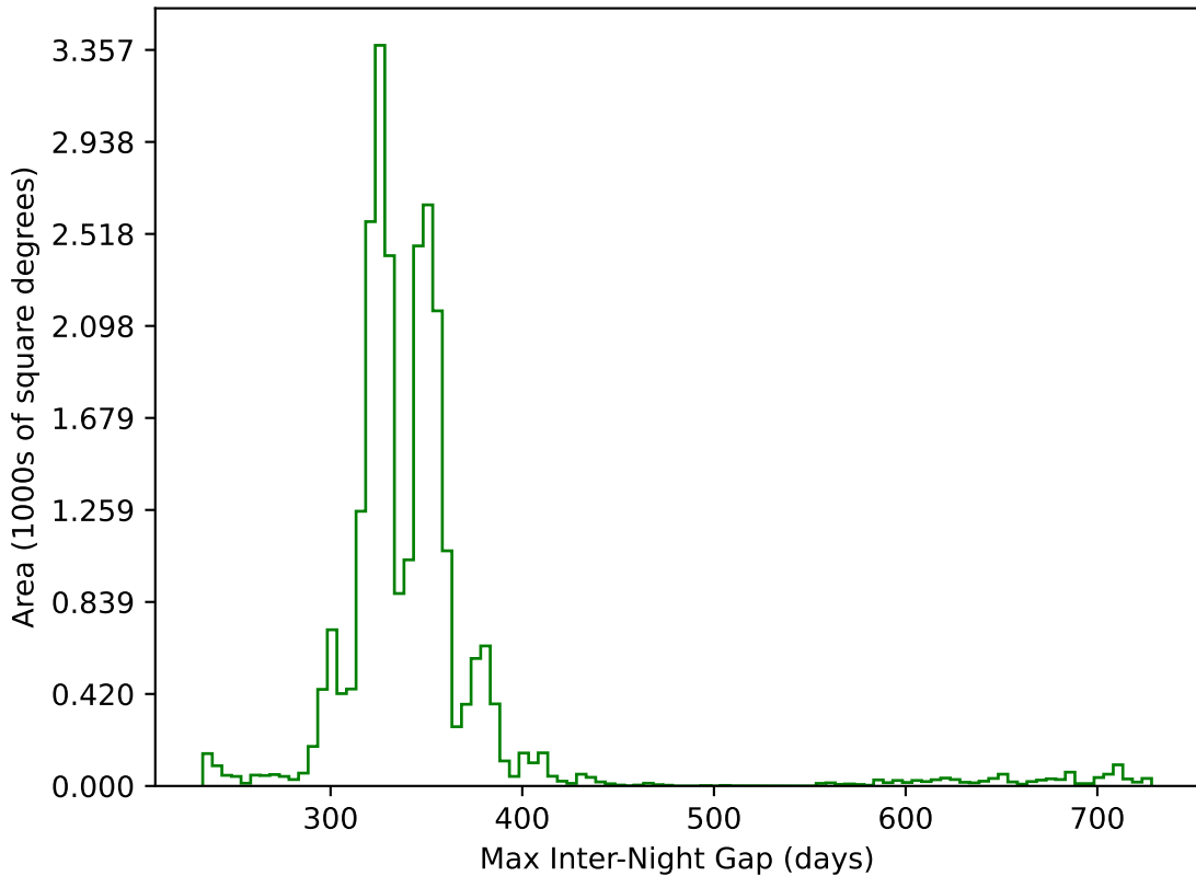
baseline_v2.1_10yrs All sky g band: Max Inter-Night Gap
