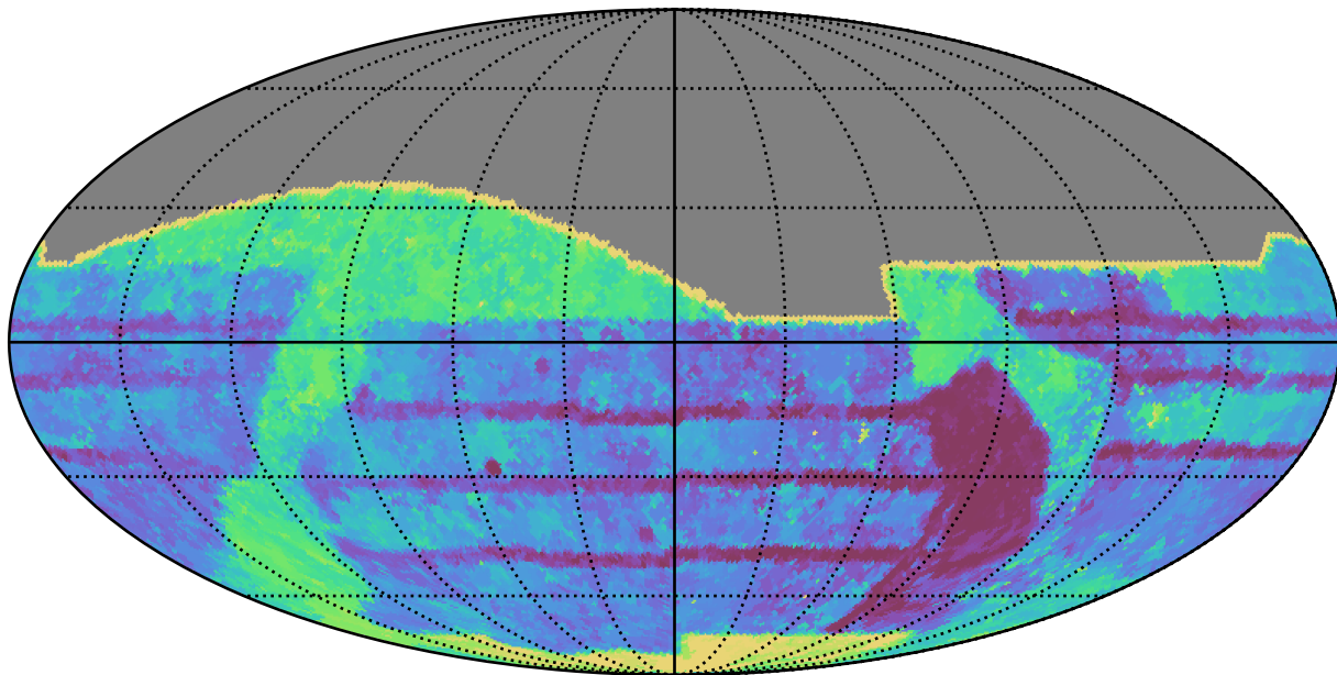
baseline_v2.1_10yrs All sky all bands: Max Inter-Night Gap
