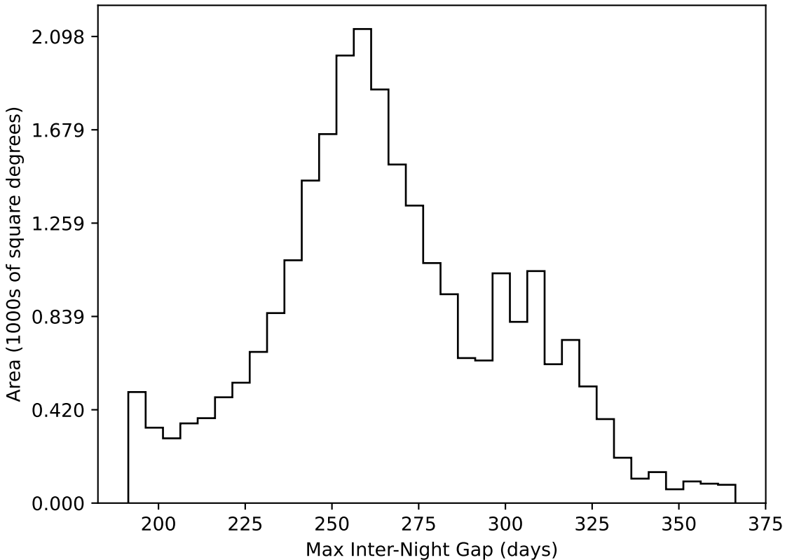
baseline_v2.1_10yrs All sky all bands: Max Inter-Night Gap
