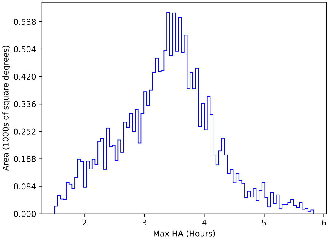
baseline_v2.1_10yrs WFD u band: Max HA
