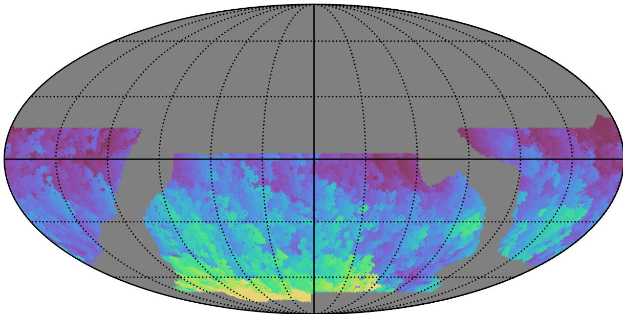
baseline_v2.1_10yrs WFD r band: Max HA
