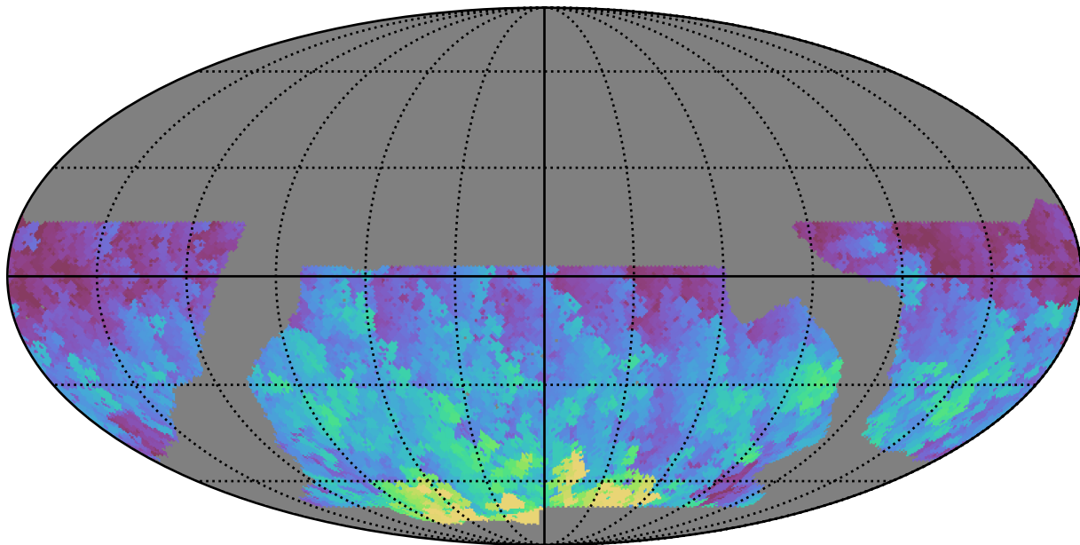
baseline_v2.1_10yrs WFD g band: Max HA
