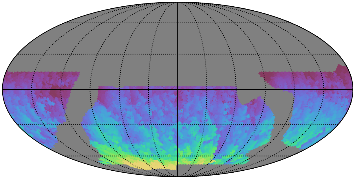
baseline_v2.1_10yrs WFD all bands: Max HA
