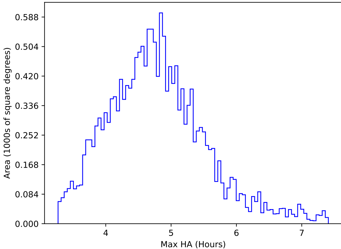
baseline_v2.1_10yrs WFD all bands: Max HA
