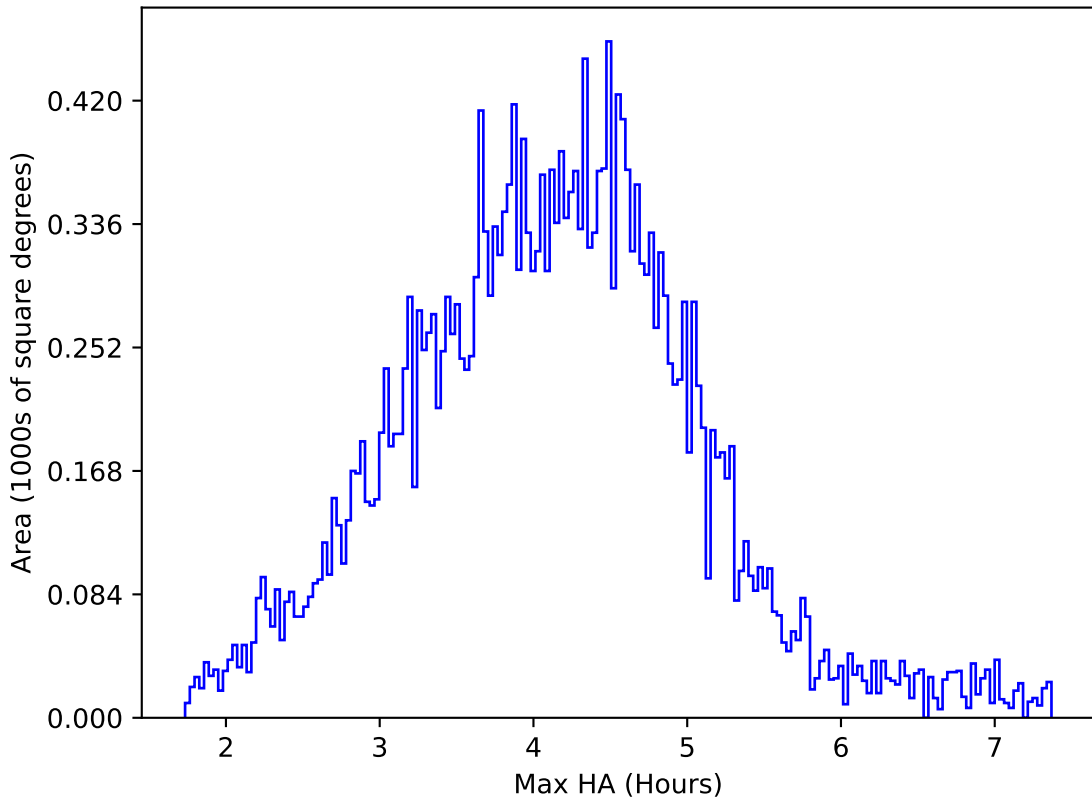
baseline_v2.1_10yrs All sky z band: Max HA
