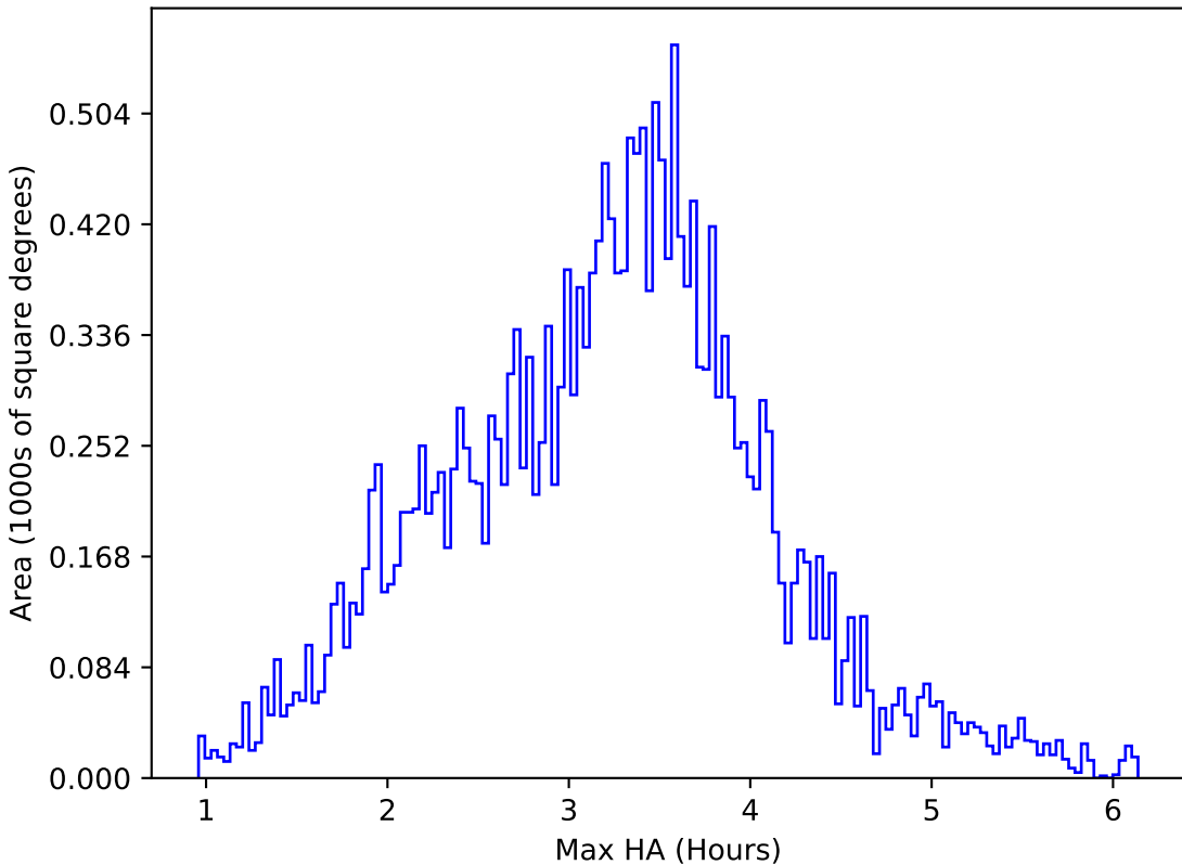
baseline_v2.1_10yrs All sky u band: Max HA
