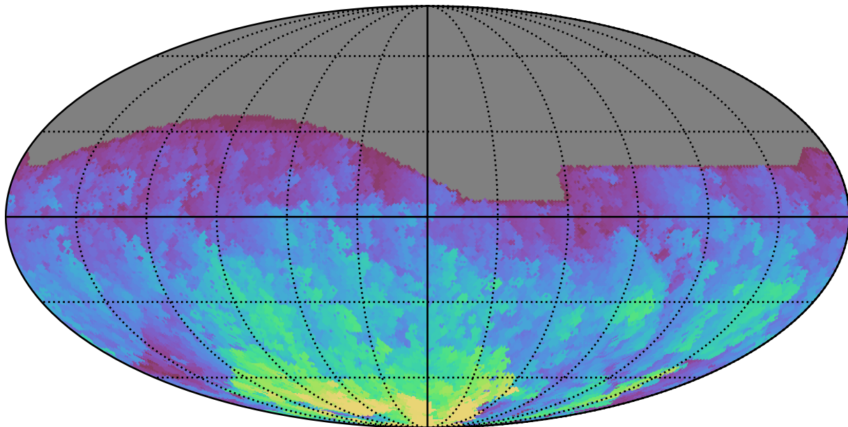
baseline_v2.1_10yrs All sky r band: Max HA
