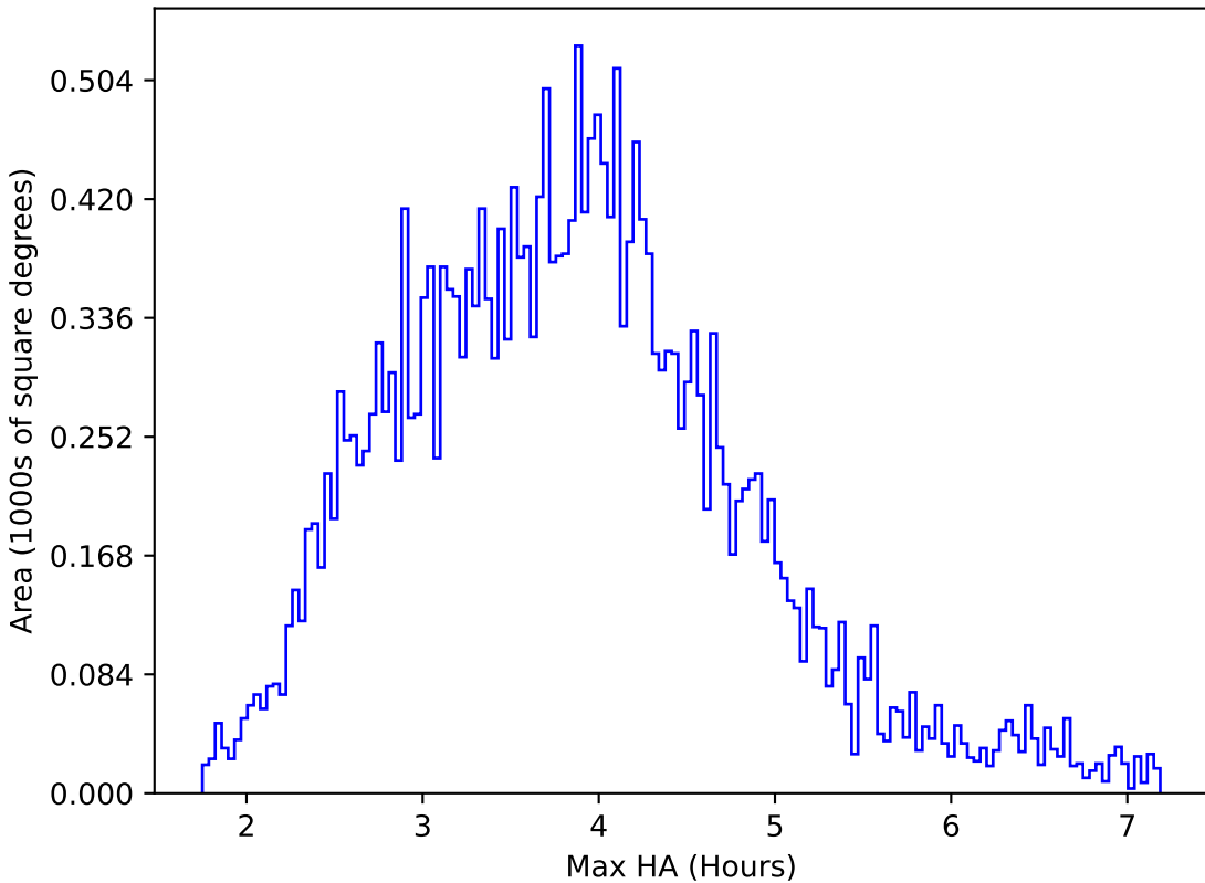
baseline_v2.1_10yrs All sky r band: Max HA
