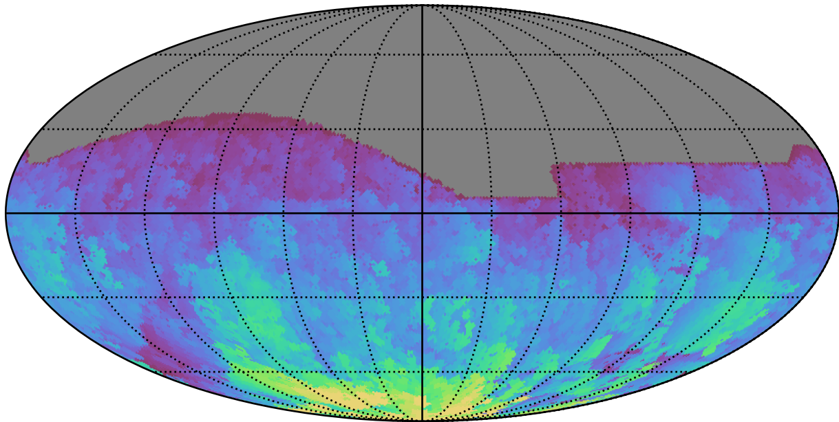
baseline_v2.1_10yrs All sky i band: Max HA
