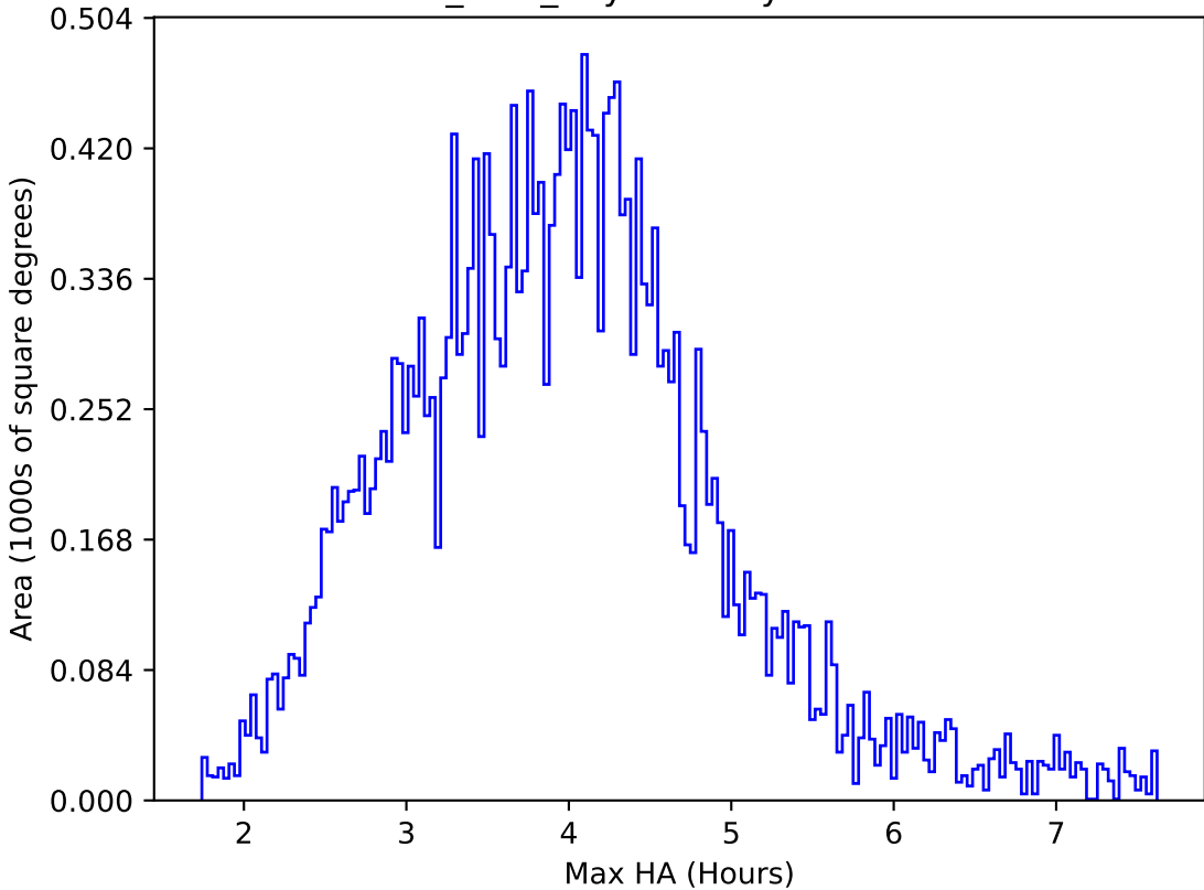
baseline_v2.1_10yrs All sky i band: Max HA
