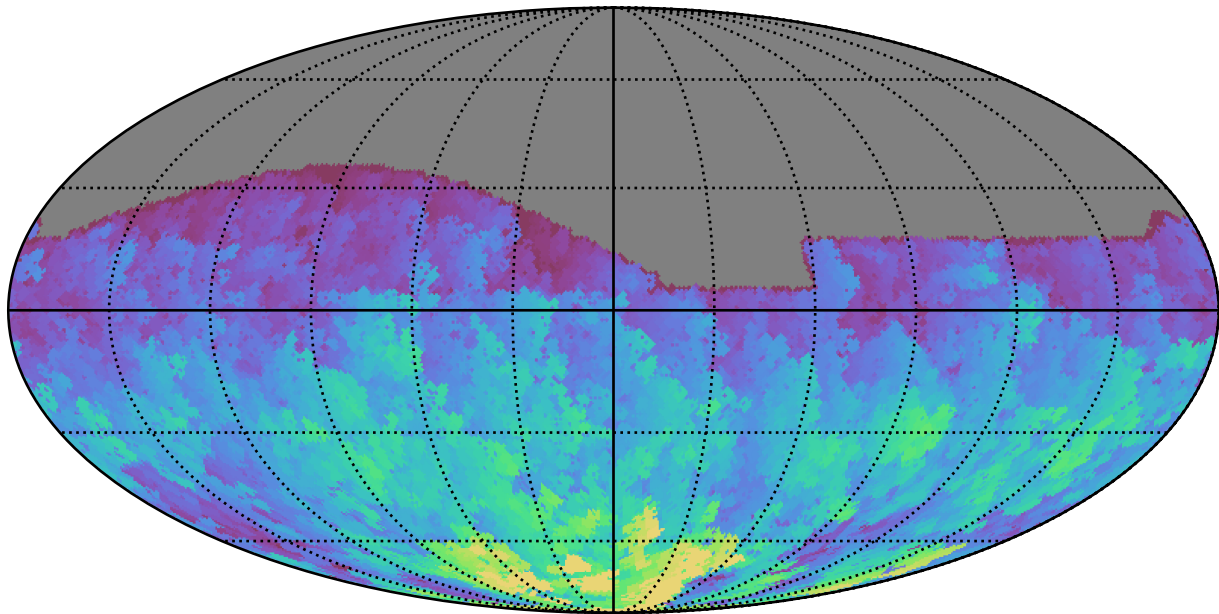
baseline_v2.1_10yrs All sky g band: Max HA
