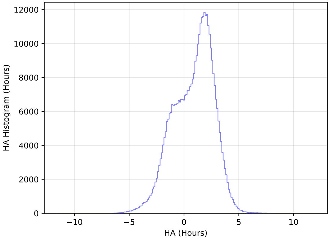
baseline_v2.1_10yrs WFD z band: HA Histogram
