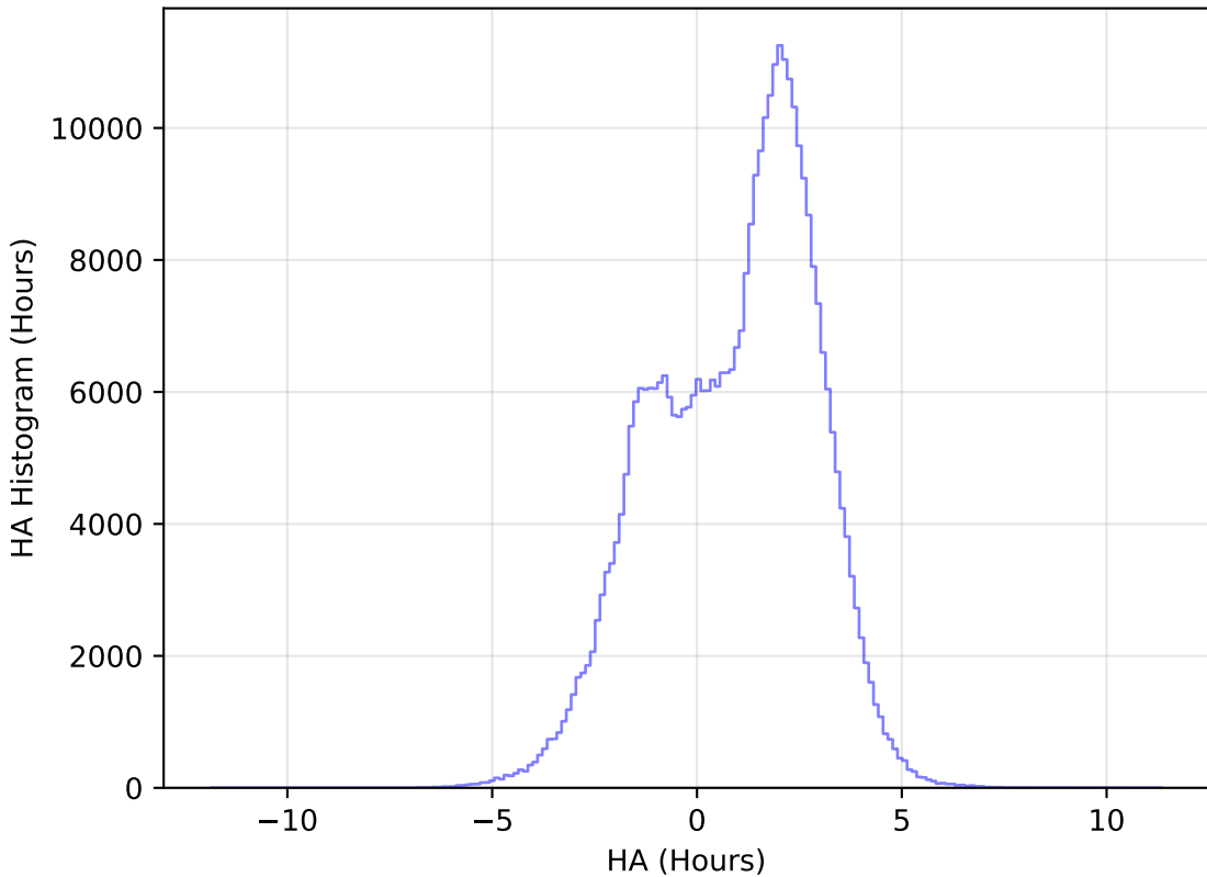
baseline_v2.1_10yrs WFD y band: HA Histogram
