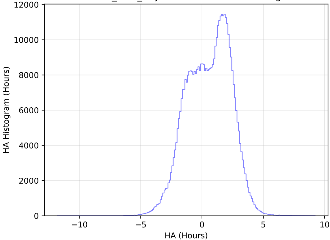
baseline_v2.1_10yrs WFD r band: HA Histogram
