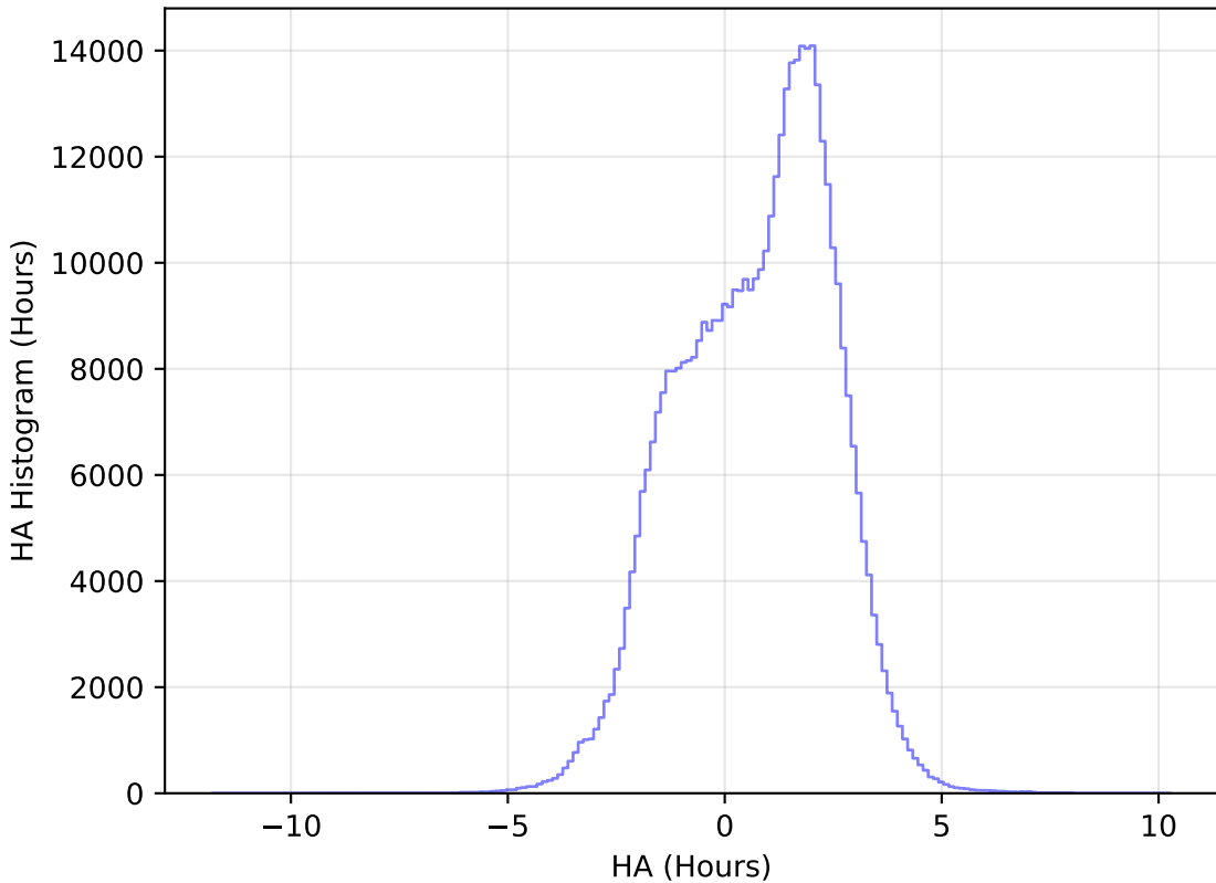
baseline_v2.1_10yrs WFD i band: HA Histogram
