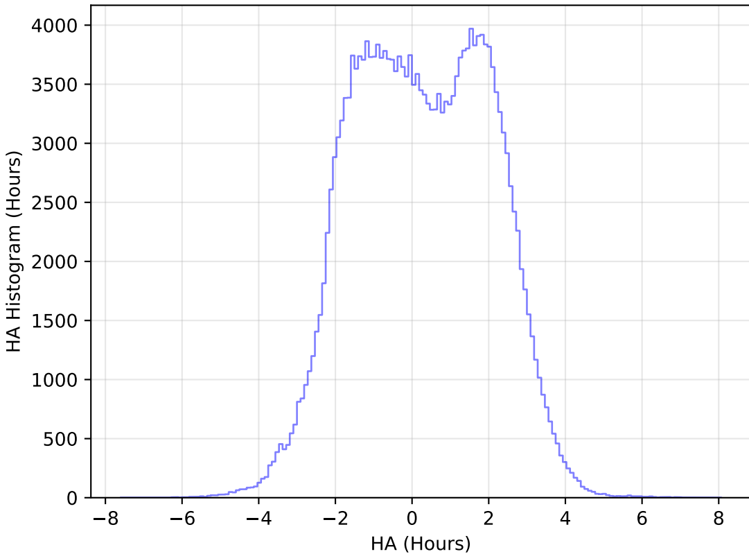
baseline_v2.1_10yrs WFD g band: HA Histogram
